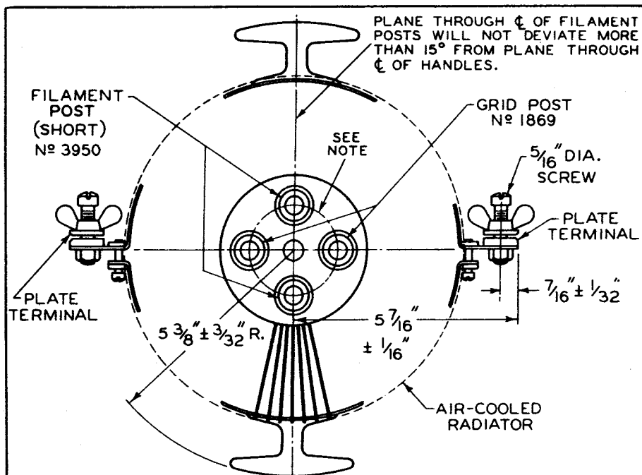
TOP VIEW OF TUBE
